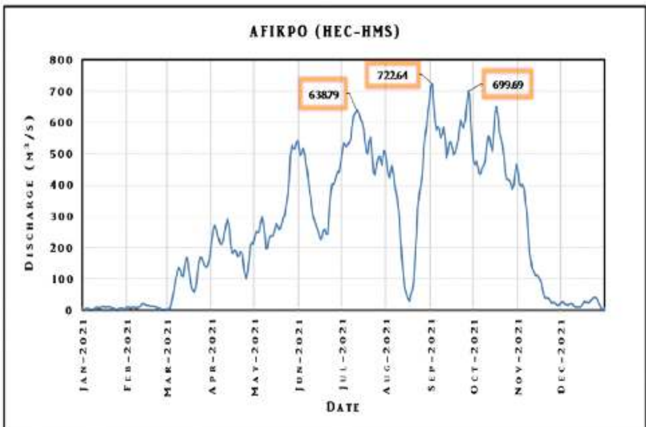
Figure 3.30: Simulated Flows at Afikpo, Cross River
