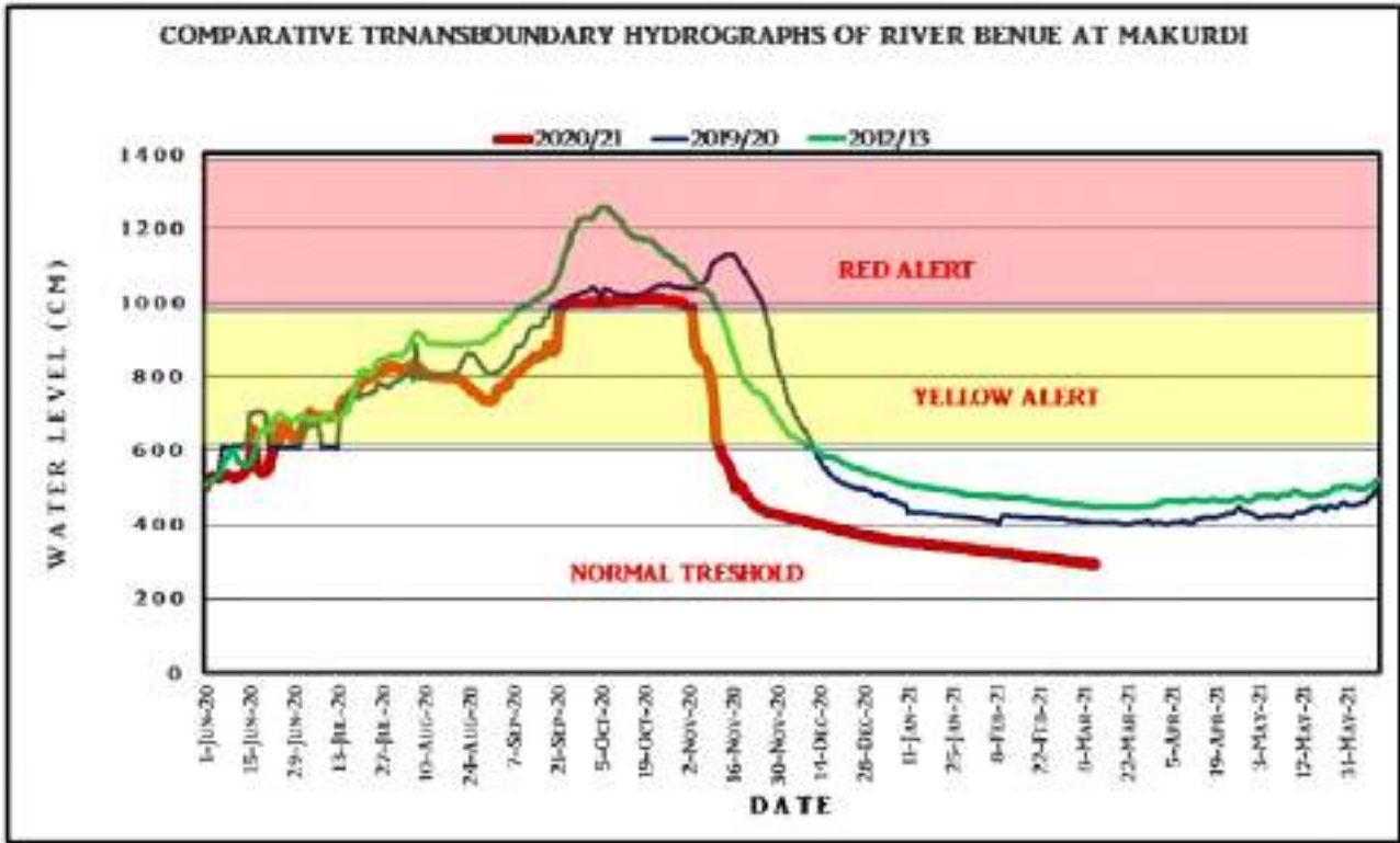
Figure 2.4: Comparative Hydrographs of River Benue at Makurdi
