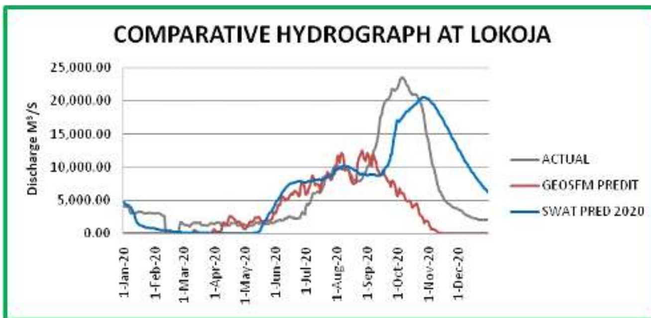
Figure 2.6 Comparative Hydrograph of Actual and Predicted Flow at Lokoja
