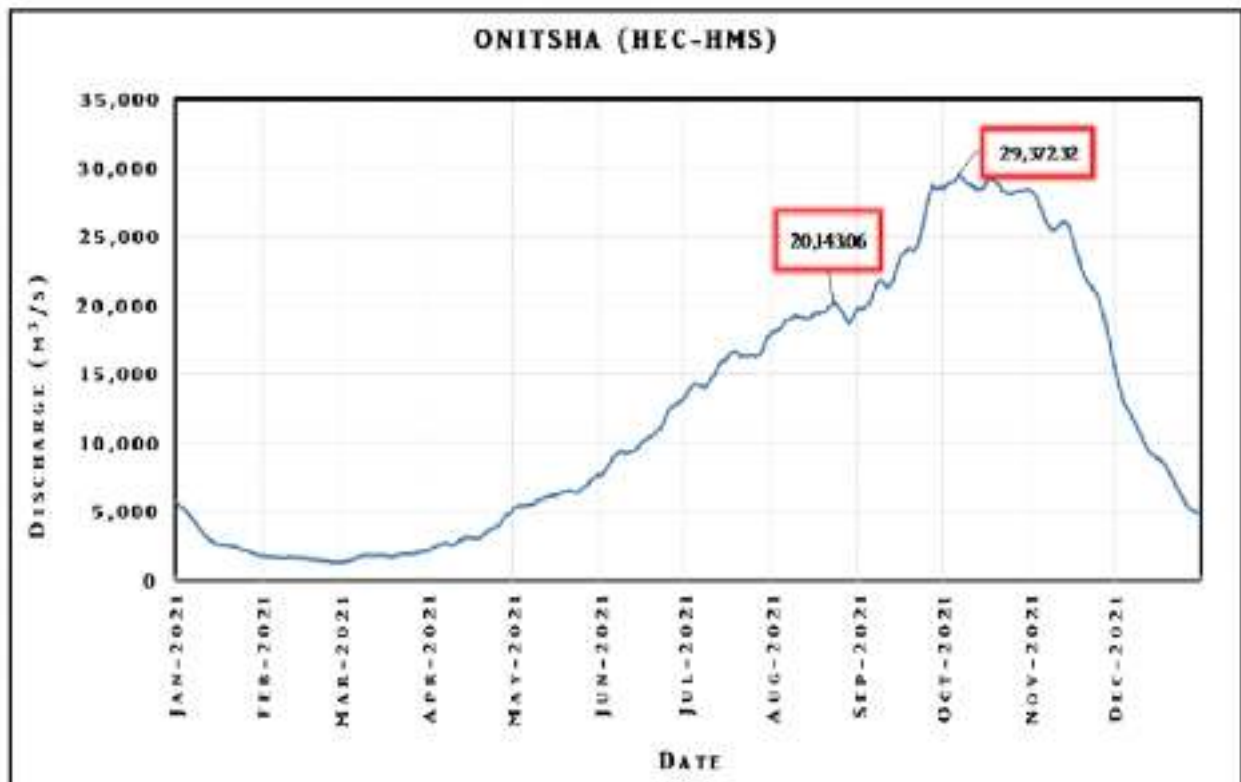
Figure 3.20: Simulated Flows at Onitsha, River Niger
