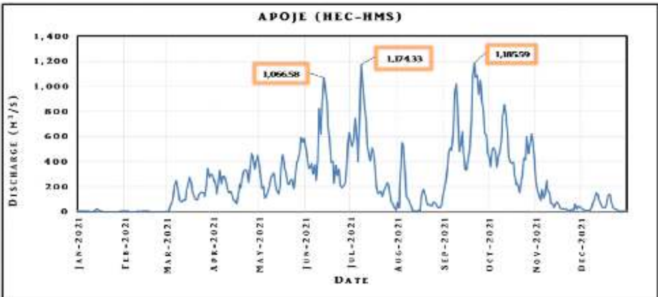
Figure 3.36: Simulated Flows at Apoje, River Oshun
