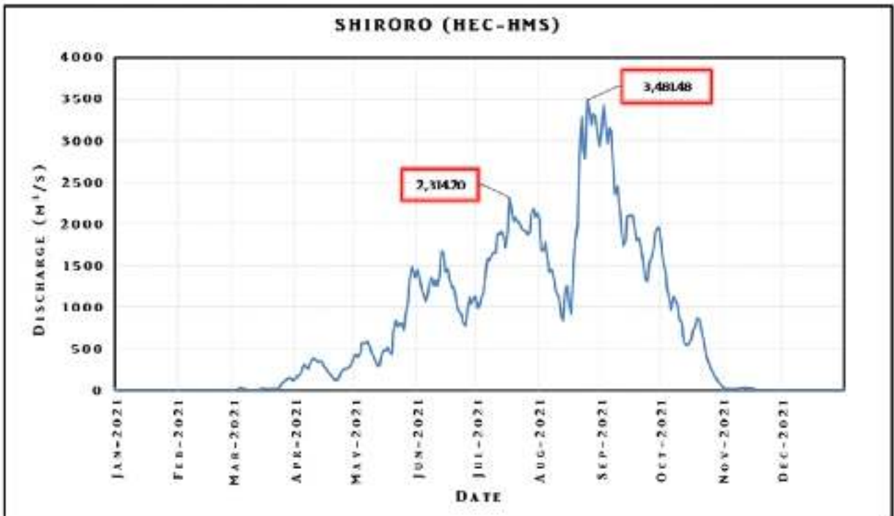
Figure 3.32: Simulated Flows at Shiroro, River Kaduna
