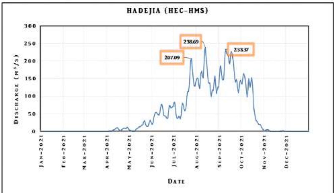
Figure 3.34: Simulated Flows at Hadejia
