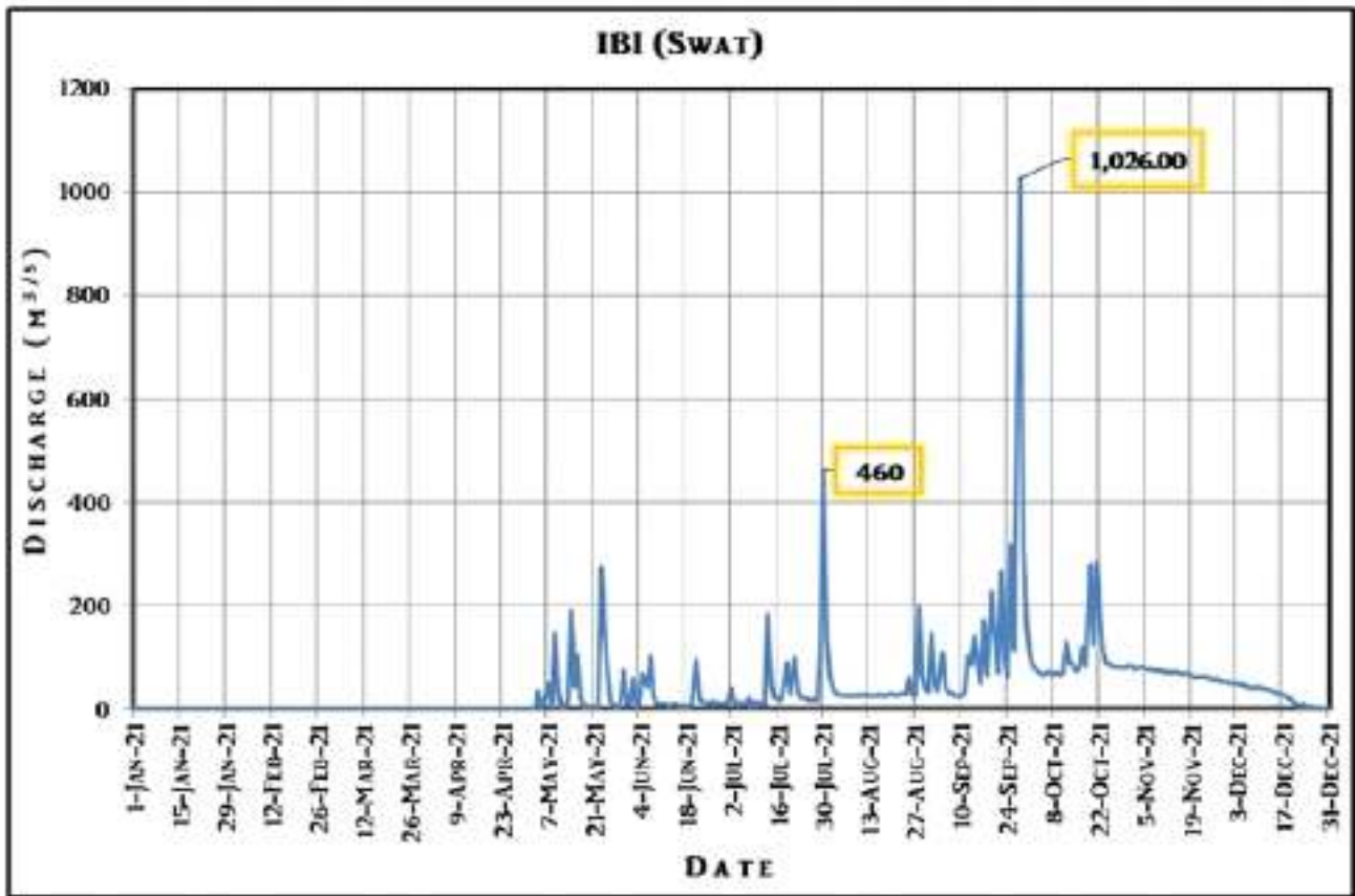
Figure 3.48: Simulated Flows at Ibi, River Ibi
