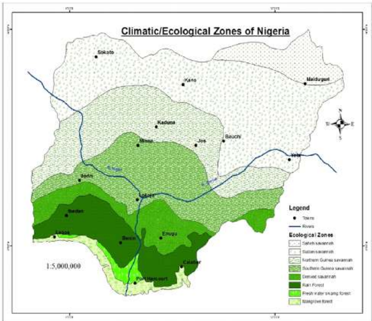
Figure 1.2: Climatic/Ecological Zones of Nigeria
