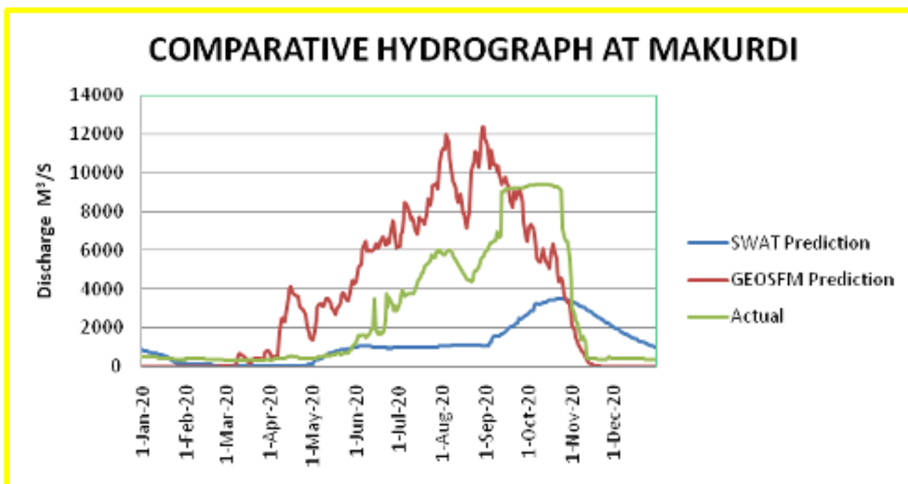
Figure 2.5. Comparative Hydrograph of Actual and Predicted Flow at Makurdi
