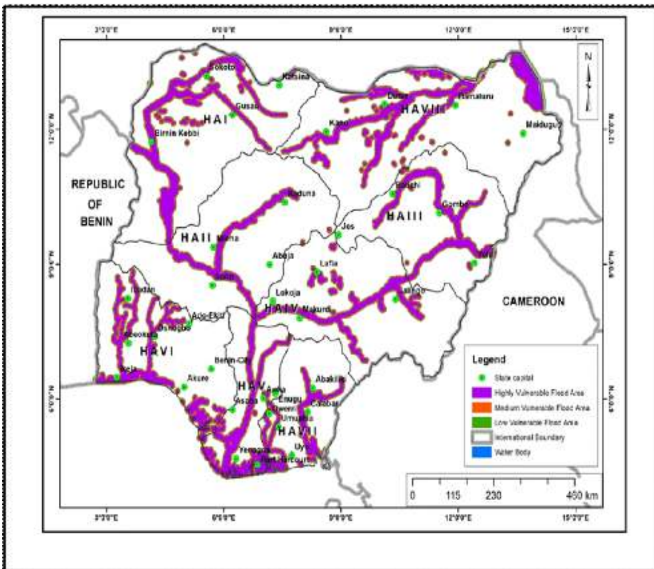
Figure 3.12: 2021 Flood Zone Vulnerability Map
