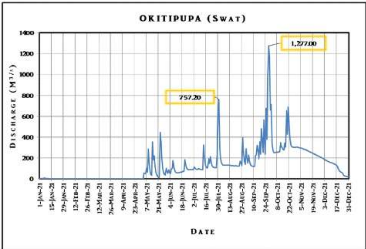
Figure 3.45: Simulated Flows at Okitipupa, River Omi Nla
